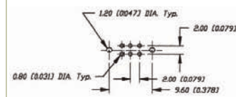
P.C. MOUNTING
